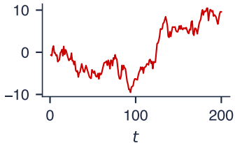
I(1) : \Delta y_t stationary
