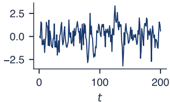
I(0) : AR(1), \phi = 0.5
