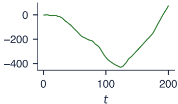
I(2) : \Delta^2 y_t stationary
