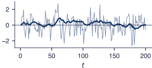
Stationary AR(1): KPSS = 0.05
