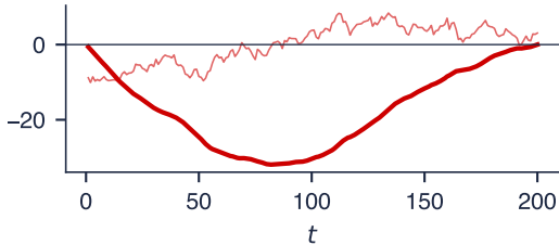
Random walk: KPSS = 1.67
