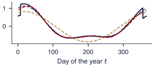
Fourier approximations with K pairs
