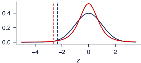
Densities of z_t , both with variance 1
