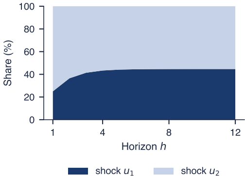
FEVD of y_2 , order (y_1, y_2)
