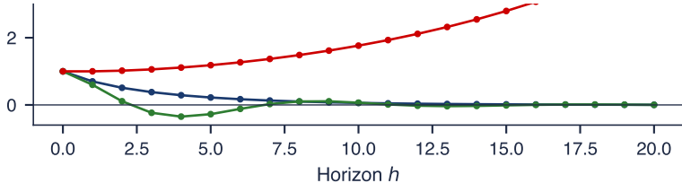
Response of y_1 to a unit shock in \varepsilon_1 , (\mathbf{A}^h)_{11}
