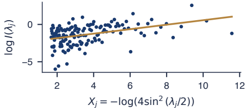
GPH regression on the first m = 142 points
