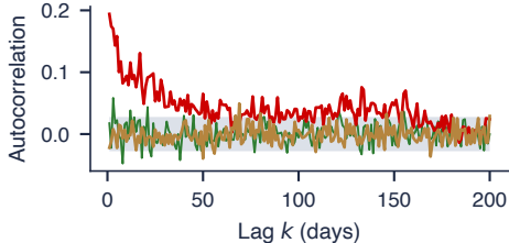
The shuffle removes the memory
