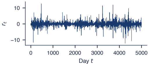
Simulated returns: calm and turbulent periods
