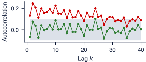
\hat{d} (LW): 0.32 before, 0.07 after
