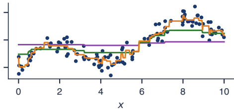
Boosting: small trees on the residuals, \nu = 0.1
