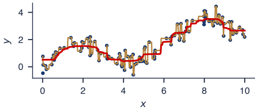
Averaging trees reduces the noise
