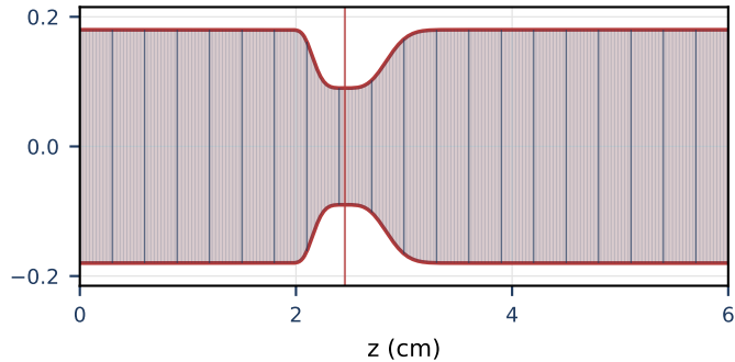
FVM cell mesh
