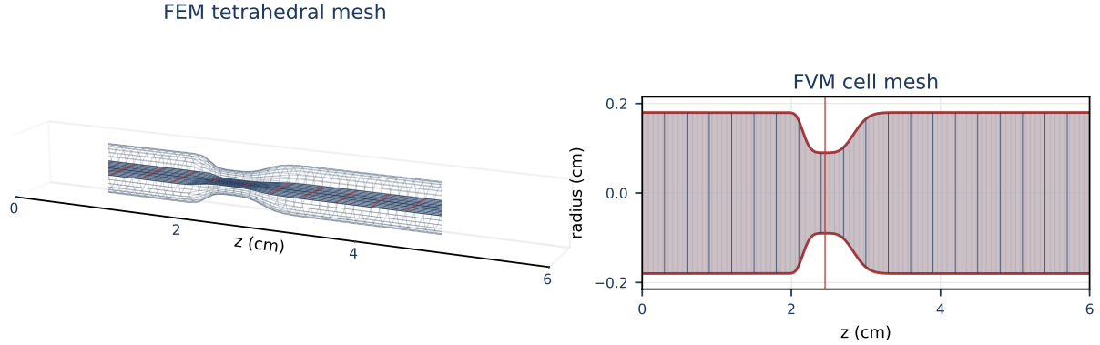
Figure 1: Finite-element and finite-volume meshes for the same smooth idealized stenosis geometry used in this report. Left: cutaway wireframe view of the generated tetrahedral Gridap mesh for the stationary-Stokes initializer. Right: one-dimensional finite-volume grid over the reference radius profile R_0(z) . The panels show discretization geometry only, not velocity, pressure-drop, pressure-ratio, or patient-specific clinical data.
