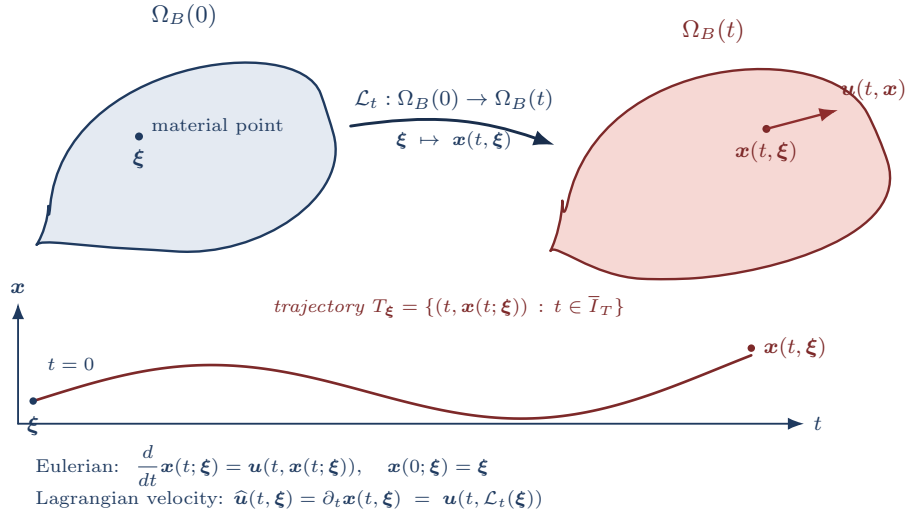
Figure 2: Lagrangian and Eulerian descriptions. The flow map \mathcal{L}_t : \Omega_B(0) \rightarrow \Omega_B(t) carries the material label \xi \in \Omega_B(0) to its current position \mathbf{x}(t, \xi) \in \Omega_B(t) . The Eulerian velocity \mathbf{u}(t, \mathbf{x}) is the velocity of whichever particle currently sits at (t, \mathbf{x}) ; the Lagrangian velocity is \hat{\mathbf{u}}(t, \xi) = \partial_t \mathbf{x}(t, \xi) = \mathbf{u}(t, \mathcal{L}_t(\xi)) , and trajectories T_{\xi} are generated by the velocity field \mathbf{u} .
