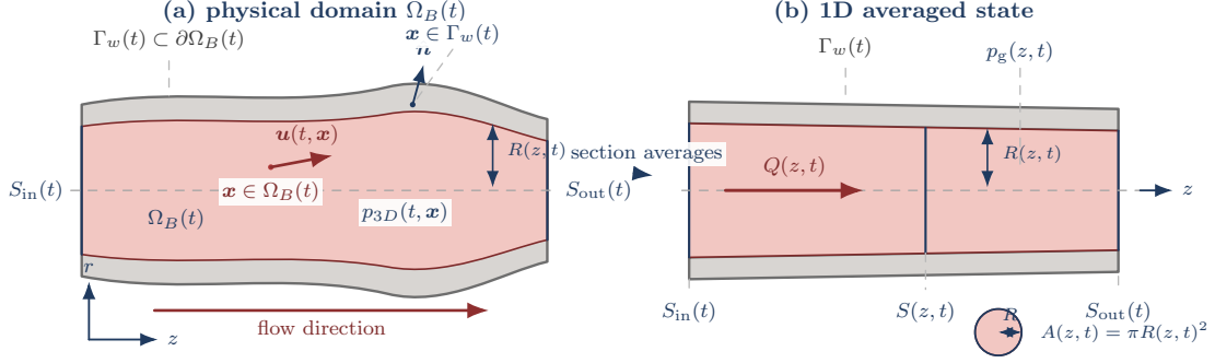
Figure 4: Compliant-vessel notation for the 1D reduction. The current configuration \Omega_B(t) is represented by a straightened averaging domain with cross-section S(z, t) , area A(z, t) , flow Q(z, t) , radius R(z, t) , and mean gauge pressure p_g(z, t) .
