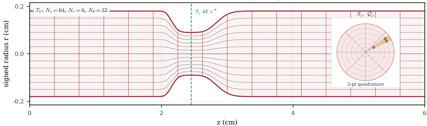
(a) FEM meridional cut and plane quadrature
