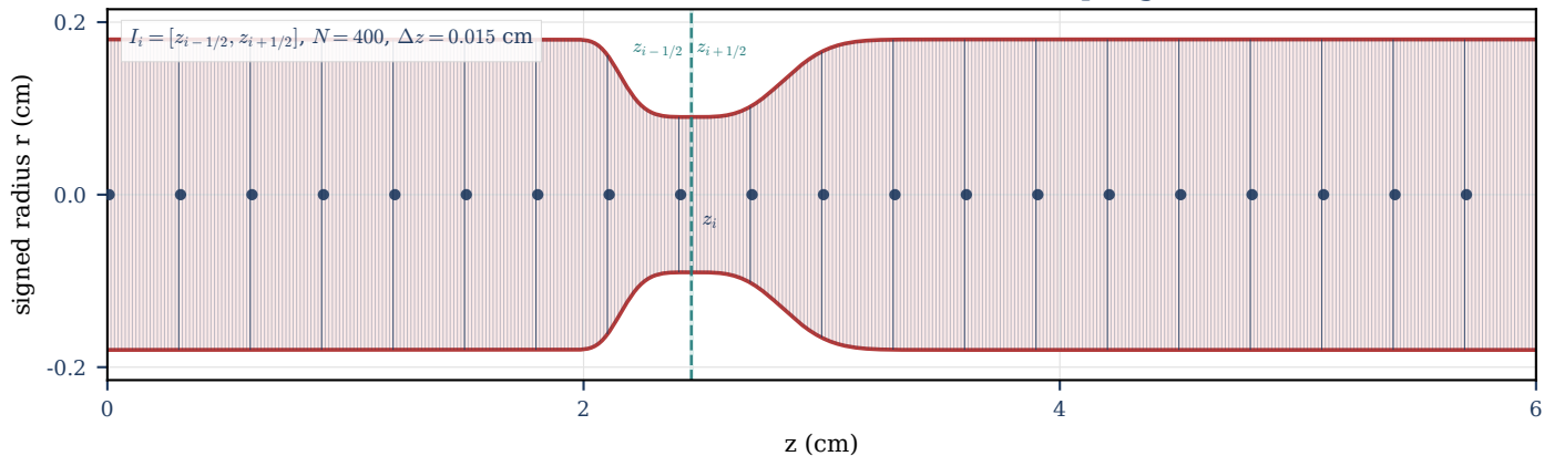
(b) FVM cells and reference-radius sampling
