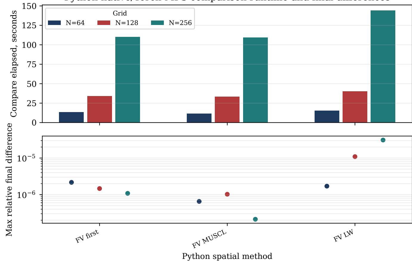
Python native/Torch-MPS comparison runtime and final differences
