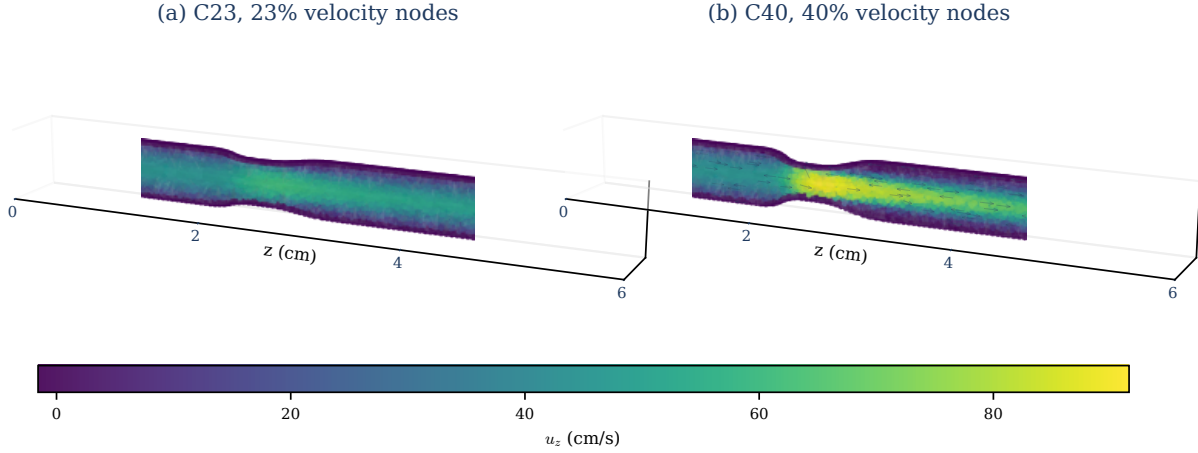
Figure 9: Resolved 3D node-centered axial velocity fields for the two T = 1 comparison cases used in Section 5. Panel (a) shows C23 with 22,691 loaded nodes; panel (b) shows C40 with 21,975 loaded nodes. The shared color scale makes the stronger axial-velocity concentration in C40 visible. Sparse arrows indicate local vector direction, and the transparent surface frames the 3D point cloud. These are resolved velocity comparison-data renderings, not the stationary-Stokes pathline proxy or a pressure-drop, FFR, or patient-specific clinical calibration measurement.
