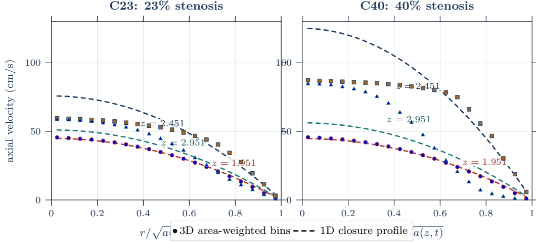
Figure 11: Radial velocity profile comparison at the declared throat-centered slices. Markers are resolved 3D area-weighted radial-bin means from the quadrature triangles; dashed curves are the 1D closure profile reconstructed from q/a . Colored in-panel labels identify the axial stations.
