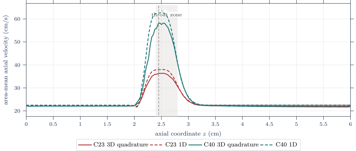
Figure 10: Area-mean axial velocity comparison at t = 1.0 s. Solid curves are tetrahedral cross-section quadrature means from the resolved 3D velocity field; dashed curves are interpolated 1D means \bar{u} = q/a = Q_{\text{phys}}/A_{\text{phys}} . The shaded band marks the throat-centered stenosis region.
