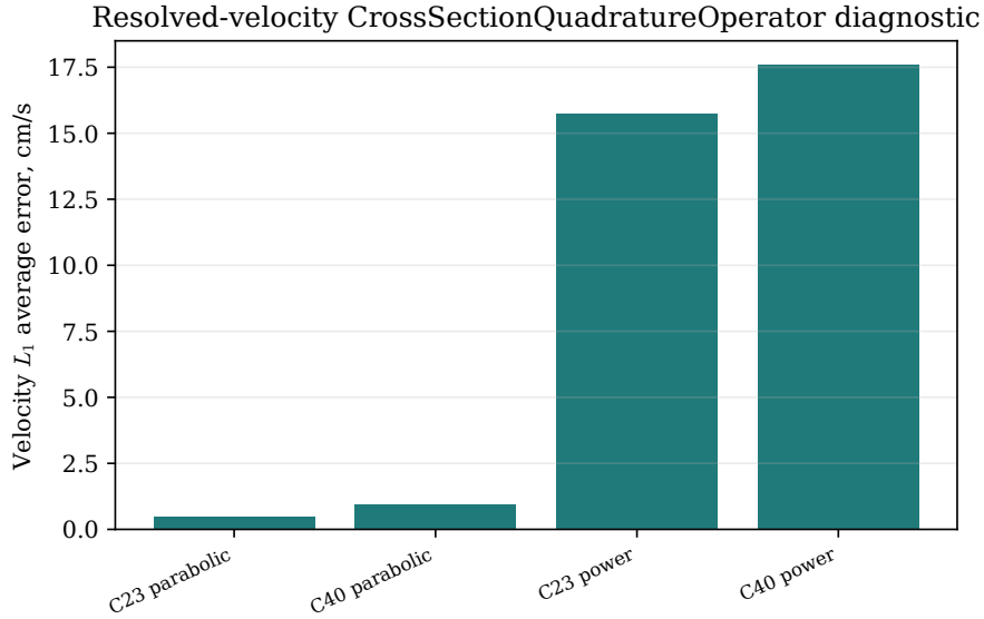
Figure 7: Resolved-velocity output-operator diagnostic summary for the available local cases. The rendered value is the section-wise mean absolute velocity discrepancy for the declared CrossSectionQuadratureOperator .
