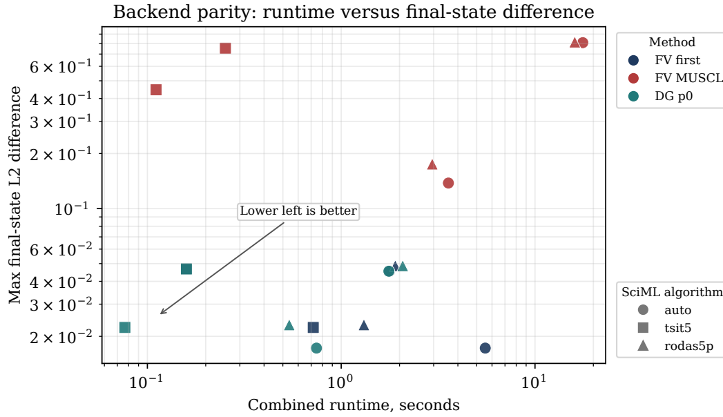
Figure 6: Native/SciML cross-integrator discrepancy versus runtime for compatible methods. The native path uses the stagewise positivity limiter; the SciML path integrates the unprojected semi-discrete system. The figure is therefore a cross-integrator diagnostic, not a proof of solver equivalence.
