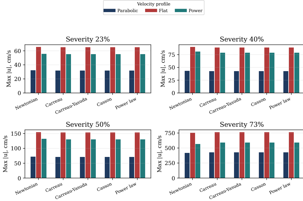
Figure 8: Rheology/profile sensitivity summary for declared descriptor combinations. This stage checks descriptor plumbing and response direction; it is not part of the principal C23/C40 comparison evidence.
