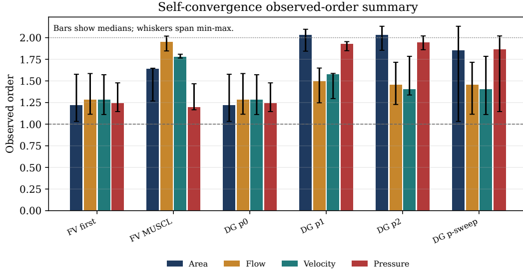
Figure 5: Self-convergence observed-order summary emitted by the benchmark renderer. This is a sampled implementation-check diagnostic; the MMS table in Section 4.2 is the stronger exact-solution verification evidence.
