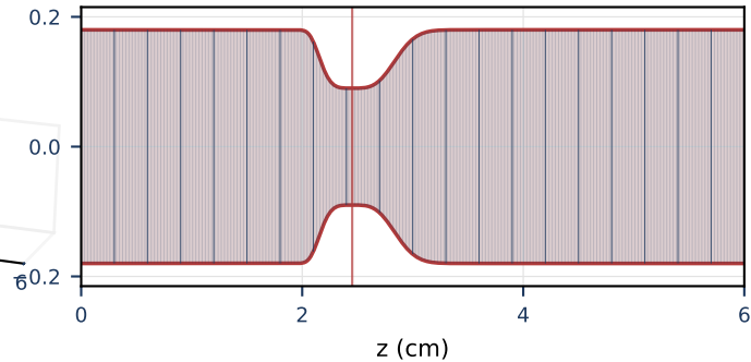
(b) FVM cell mesh
