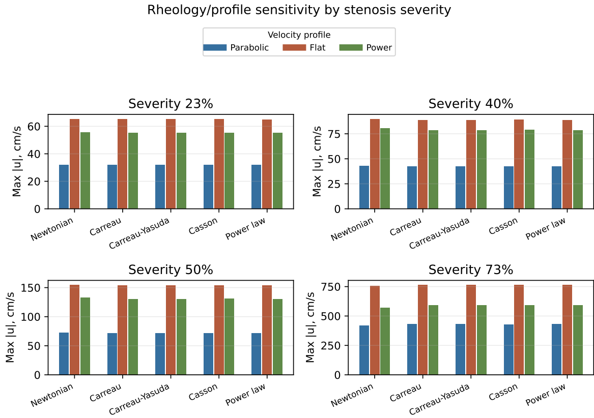
Figure 13: Rheology/profile sensitivity summary for declared descriptor combinations. Facets separate stenosis severity; grouped bars separate the rheology and velocity-profile descriptors. The diagnostic shows how the maximum speed responds to descriptor choices within the emitted benchmark records.
