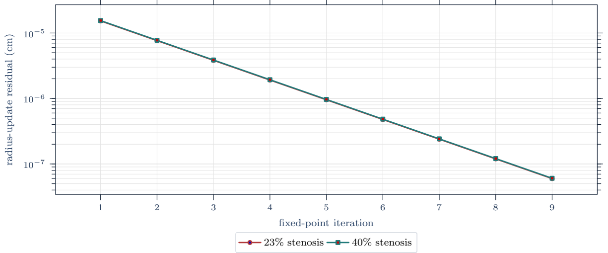
Figure 9: Fixed-point convergence for the quasi-static membrane-FSI comparator. The residual is the maximum radial-radius update between successive coupled wall solves, reported in centimeters; it checks the comparator solve, not the 1D–3D velocity observation error.
