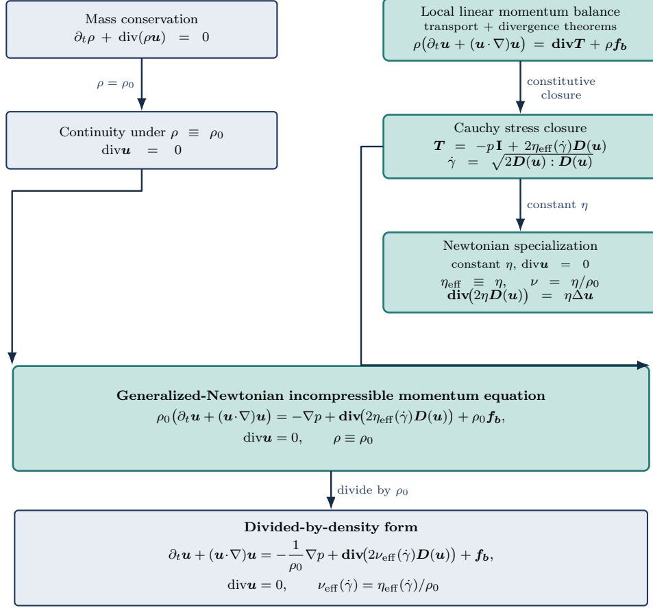
Figure 2: From conservation laws to incompressible Navier–Stokes. Mass conservation reduces to \text{div} \mathbf{u} = 0 under constant density. Momentum balance closes through the Cauchy stress law; the Newtonian limit uses constant dynamic viscosity, while the generalized-Newtonian form keeps \eta_{\text{eff}}(\dot{\gamma}) explicit.
