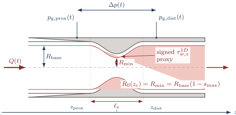
Figure 6: Schematic tap and output convention for an idealized stenosis, not drawn from a computed case. The taps define \Delta p(t) ; \pi_{\text{PR}} additionally declares the averaging window, pressure reference, and denominator rule needed for \text{PR}_{1D}(\pi_{\text{PR}}) .
