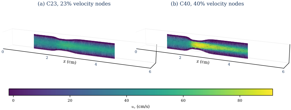
Figure 4: Final-time resolved velocity samples used by the 23% and 40% stenosis comparisons. The panels show node-centered u_z values; the quantitative comparison enters only after applying the declared cross-sectional observation operator.
