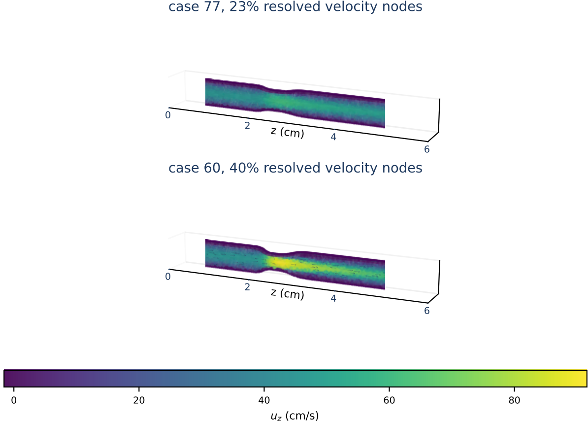
Figure 4: Resolved 3D node-centered axial velocity fields for the two T = 1 comparison cases used in Section 2. The panels show deterministic half-domain cutaway views of the full upstream XDMF/HDF5 velocity fields: case 77 has 22,691 loaded nodes and case 60 has 21,975 loaded nodes. Color denotes u_z in cm/s, sparse arrows indicate local vector direction, and the transparent surface is the node envelope used only to frame the 3D point cloud. These are resolved velocity-data renderings, not the stationary-Stokes pathline proxy or a pressure-drop, FFR, or patient-specific clinical calibration measurement.
