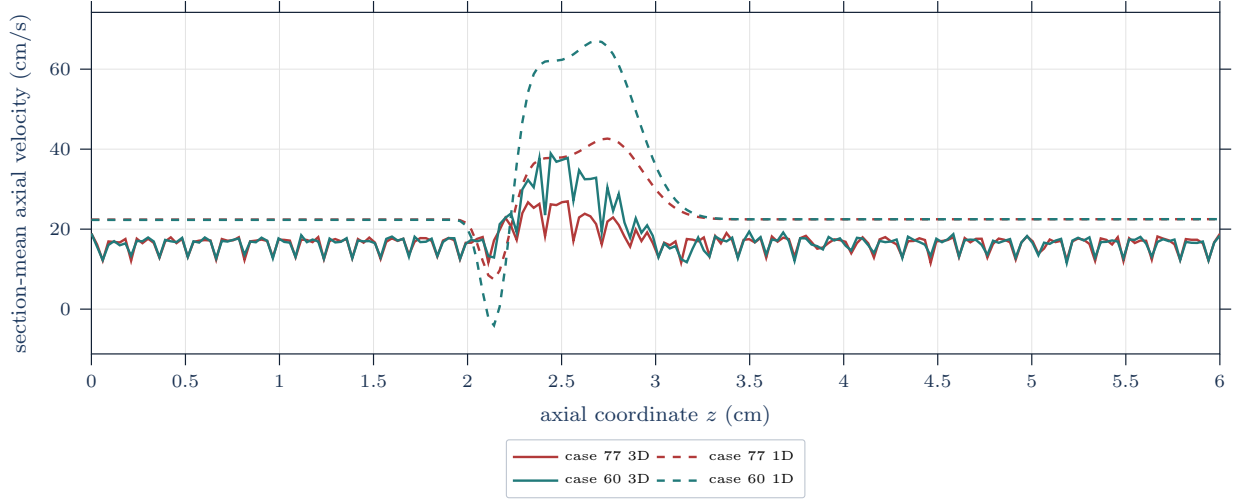
Figure 9: Section-mean axial velocity comparison at T = 1 . Solid curves are resolved 3D node-slab means; dashed curves are interpolated 1D Q/A .
