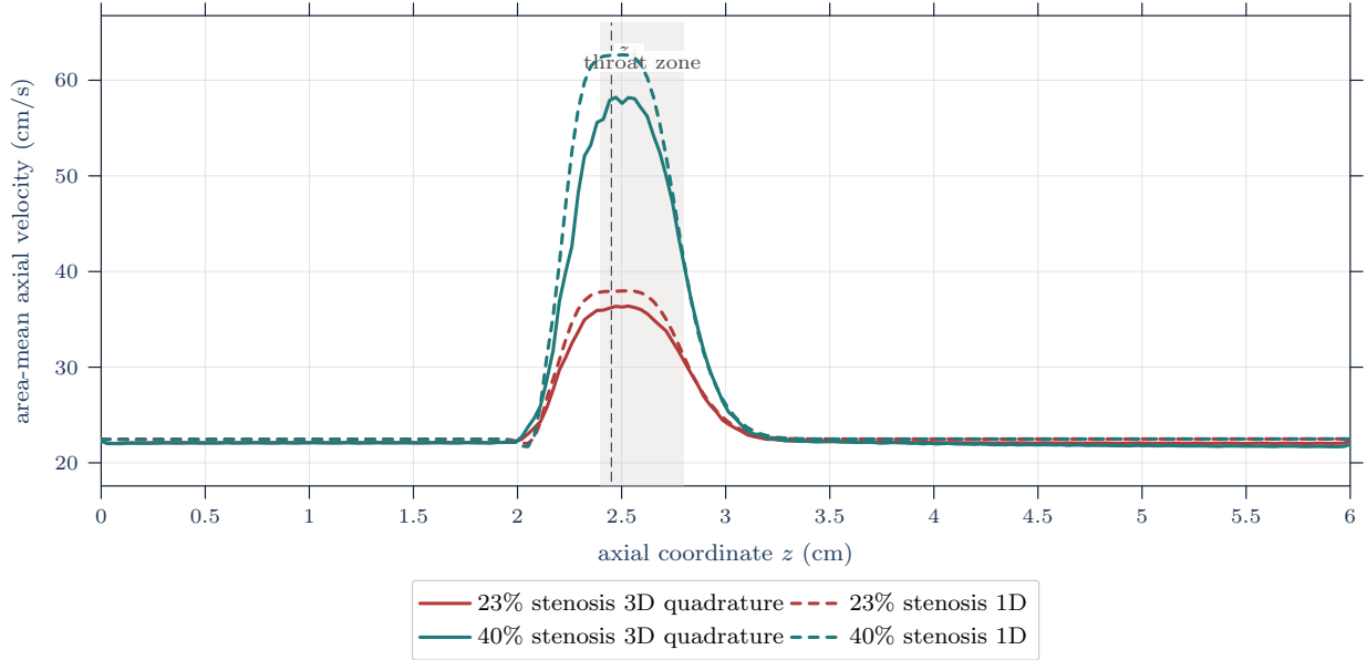
Figure 5: Area-mean axial velocity comparison at t = 0.9995 s under the reference-coordinate section observation map. Solid curves are tetrahedral cross-section quadrature means from the resolved 3D velocity field; dashed curves are interpolated 1D means \bar{u} = q/a = Q_{\text{phys}}/A_{\text{phys}} .
