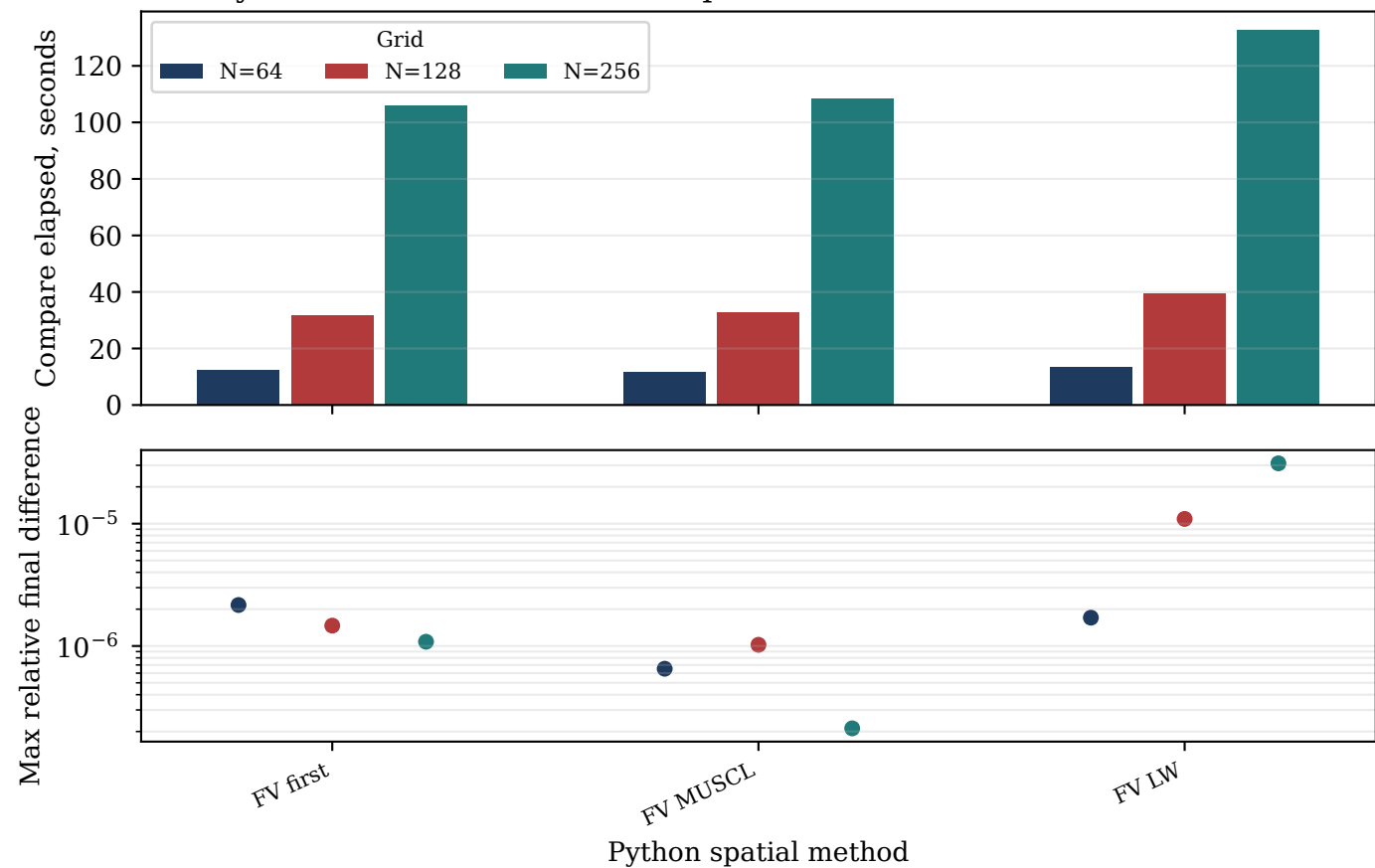
Python native/Torch-MPS comparison runtime and final differences
