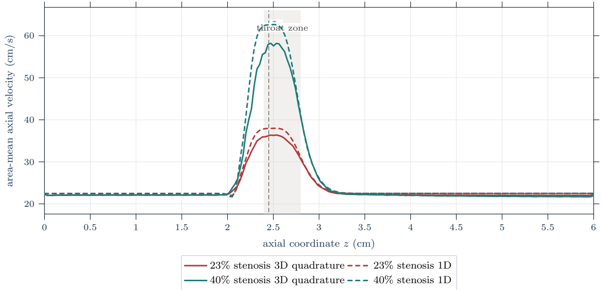
Figure 5: Area-mean axial velocity comparison at t = 0.9995 \text{ s} under the reference-coordinate section observation operator. Solid curves are tetrahedral cross-section quadrature means from the resolved 3D velocity field; dashed curves are interpolated 1D means \bar{u} = q/a = Q_{\text{phys}}/A_{\text{phys}} .
