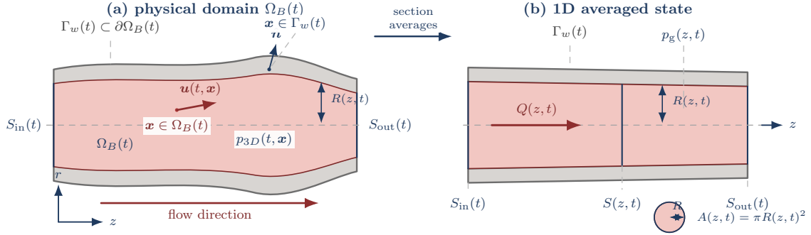
Figure 5: Compliant-vessel notation for the 1D reduction. The current configuration \Omega_B(t) is represented by a straightened averaging domain: section averages over S(z, t) define A(z, t) , Q(z, t) , \bar{u}(z, t) , and p_g(z, t) , while R(z, t) records the radius entering the wall and geometry closures. The figure is a bookkeeping reduction from continuum fields to retained 1D variables, not a resolved wall-traction or secondary-flow model.
