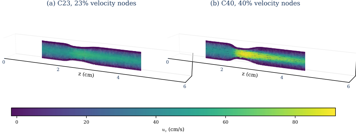
Figure 13: Resolved 3D node-centered axial velocity fields for the two T = 1 comparison cases used in Section 2. Panel (a) shows C23 with 22,691 loaded nodes; panel (b) shows C40 with 21,975 loaded nodes. The shared color scale makes the stronger axial-velocity concentration in C40 visible. Sparse arrows indicate local vector direction, and the transparent surface frames the 3D point cloud. These are resolved velocity-data renderings, not the stationary-Stokes pathline proxy or a pressure-drop, FFR, or patient-specific clinical calibration measurement.
