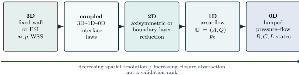
Figure 4: Model hierarchy for reading comparison claims, ordered from the three-dimensional continuum tier toward reduced and lumped closures. The horizontal direction is a dimensional-reduction and closure-abstraction axis, not a validation ranking. This report selects a 1D reduced forward model; 3D fixed-wall, resolved FSI, clinical, and independent-solver comparisons require separately matched assumptions, inputs, output operators, and discrepancy metrics before they can support evidence claims.
