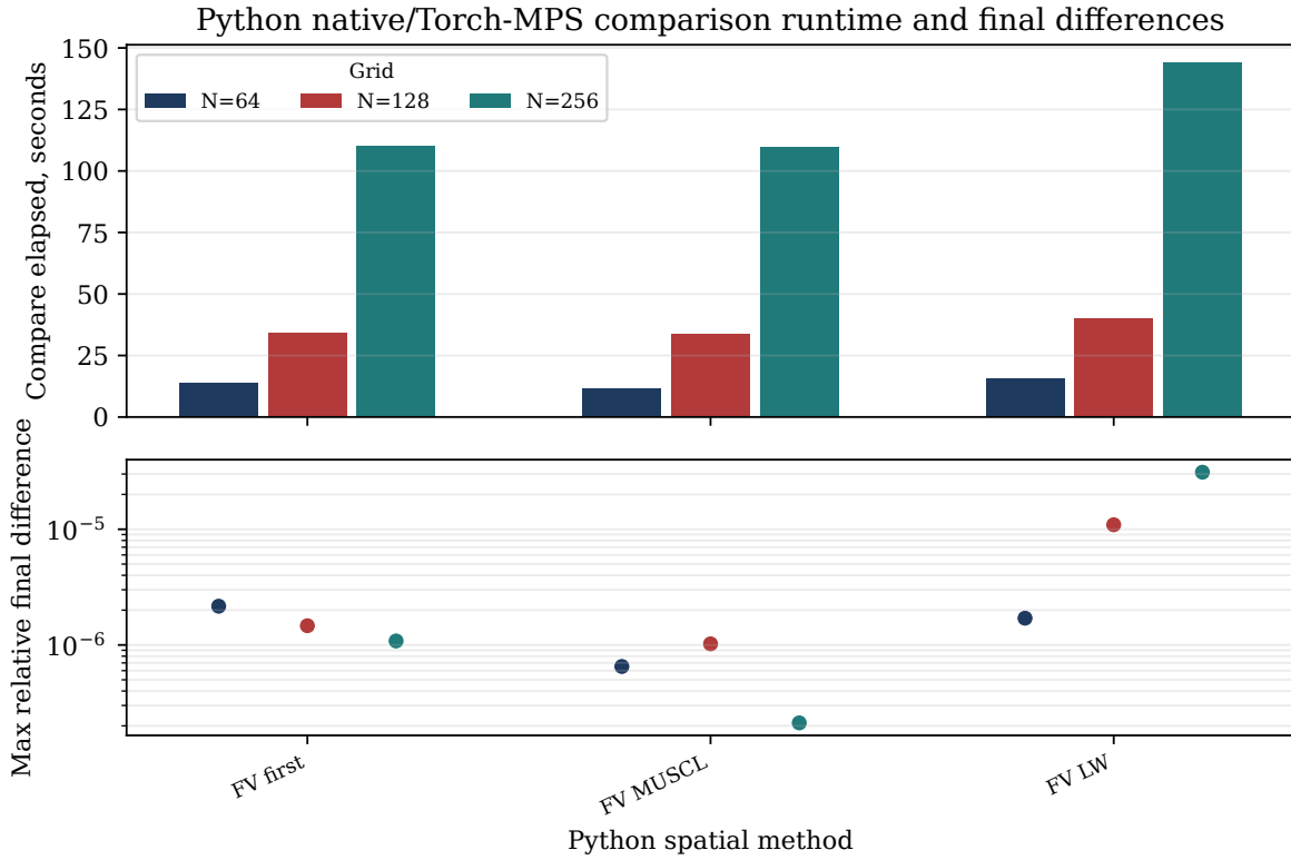
Figure 15: Python native CPU versus Torch-MPS comparison for the Python CLI surface. The top panel reports elapsed time by method and grid size; the lower panel reports the maximum relative final-state difference across the emitted area and flow summaries.
