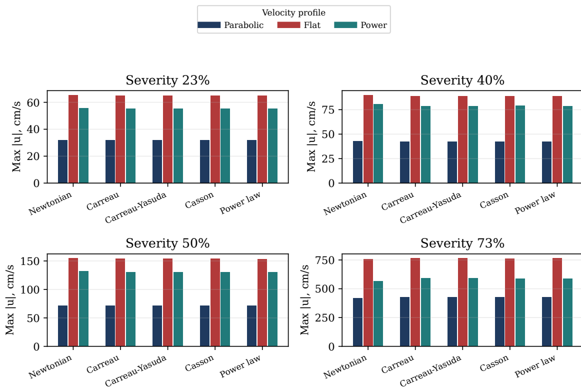
Figure 13: Rheology/profile sensitivity summary for declared descriptor combinations. Facets separate stenosis severity; grouped bars separate the rheology and velocity-profile descriptors. The diagnostic shows how the maximum speed responds to descriptor choices within the emitted benchmark records.
