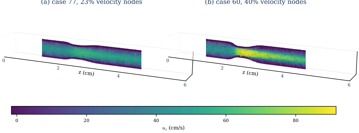
Figure 5: Resolved 3D node-centered axial velocity fields for the two T = 1 comparison cases used in Section 2. Panel (a) shows case 77 with 22,691 loaded nodes; panel (b) shows case 60 with 21,975 loaded nodes. The shared color scale makes the stronger axial-velocity concentration in the 40% case visible. Sparse arrows indicate local vector direction, and the transparent surface frames the 3D point cloud. These are resolved velocity-data renderings, not the stationary-Stokes pathline proxy or a pressure-drop, FFR, or patient-specific clinical calibration measurement.
