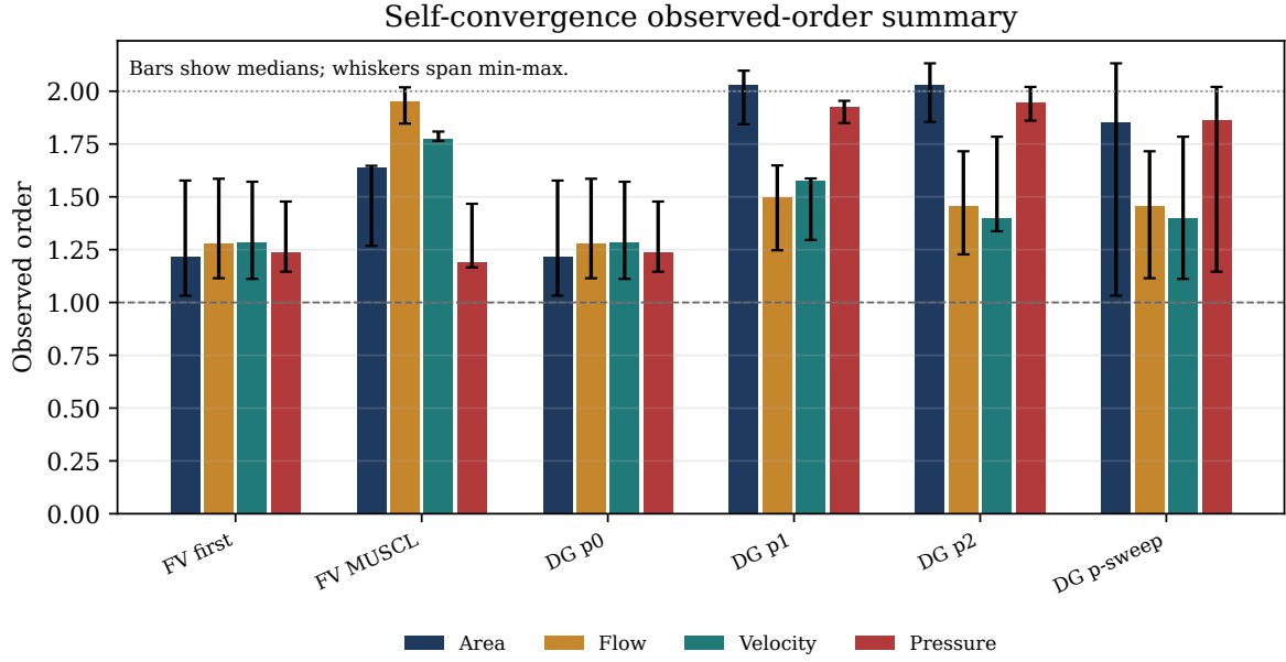
Figure 11: Self-convergence observed-order summary emitted by the package benchmark renderer. Bars report median observed order by method and metric; whiskers show the observed min-max range across the benchmarked refinements. This is an internal convergence diagnostic, not external validation evidence.
