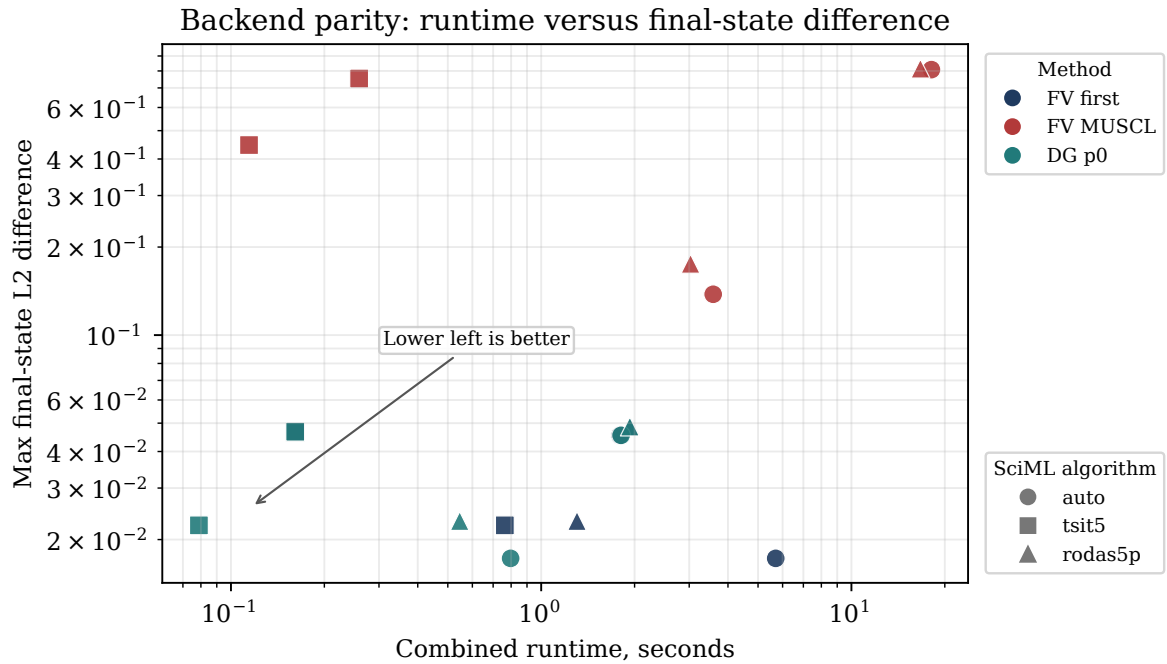
Figure 12: Native/SciML backend agreement versus runtime for benchmarked compatible methods. Color identifies the method family, marker shape identifies the SciML algorithm, and lower-left points are both faster and closer to the native final state under the plotted aggregate difference.
