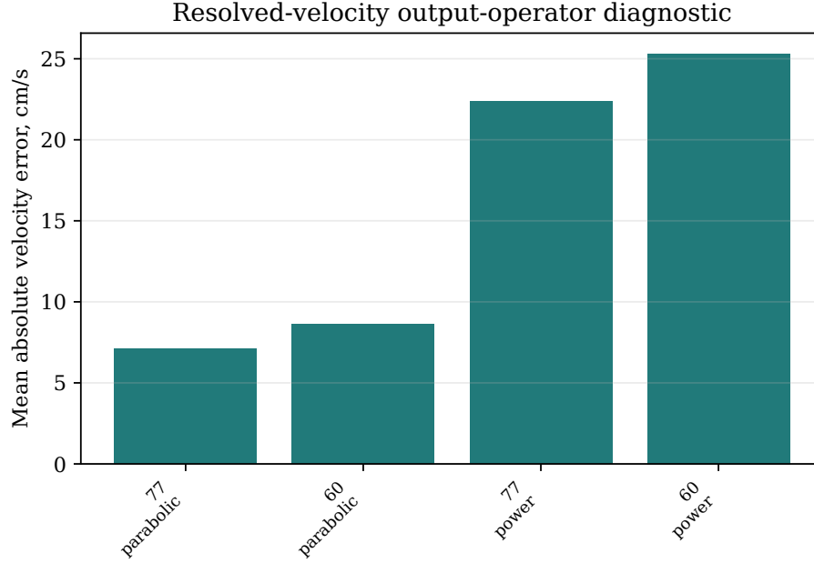
Figure 14: Resolved-velocity output-operator diagnostic summary for the available local cases. The package-benchmark CSVs contain four OK resolved-velocity rows across the parabolic and power-profile closures; the panel remains an output-operator diagnostic rather than a resolved-3D validation claim.
