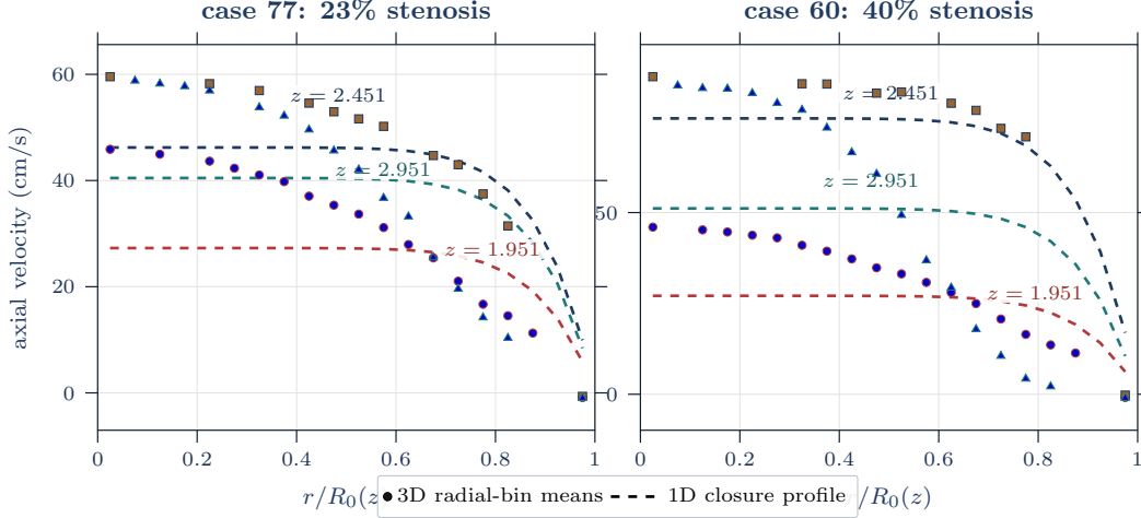
Figure 10: Radial velocity profile comparison at the declared throat-centered slices. Markers are resolved 3D radial-bin means; dashed curves are the 1D closure profile reconstructed from Q/a . Colored in-panel labels identify the axial stations, making the downstream case-60 discrepancy visible without repeating a separate legend in each panel.
