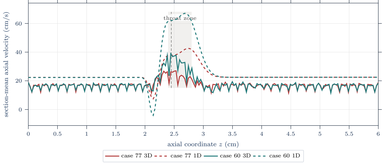
Figure 9: Section-mean axial velocity comparison at T = 1 . The shaded band marks the throat-centered stenosis region near z_* ; solid curves are resolved 3D node-slab means, and dashed curves are interpolated 1D Q/a , equivalently Q_{\text{phys}}/A_{\text{phys}} under the declared \pi -scaling. The mismatch localizes near the stenosis and is larger for the 40% case.
