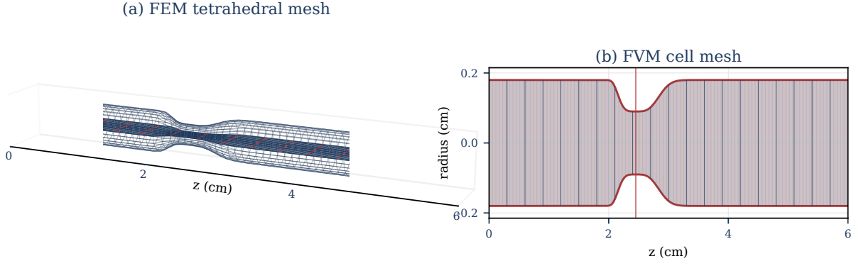
Figure 1: Finite-element and finite-volume views of the same smooth idealized stenosis geometry used in this report. Panel (a) shows the generated tetrahedral Gridap mesh for the stationary-Stokes initializer; panel (b) shows the one-dimensional finite-volume grid sampled along the reference radius profile R_0(z) . The takeaway is that one declared geometry can feed distinct discretizations; the panels show geometry only, not velocity, pressure-drop, pressure-ratio, or patient-specific clinical data.
