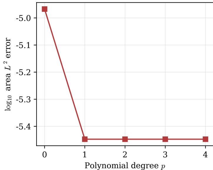
Fixed-mesh p sweep
