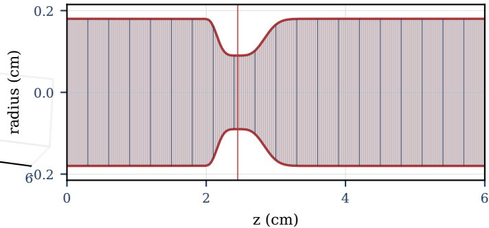
(b) FVM cell mesh
