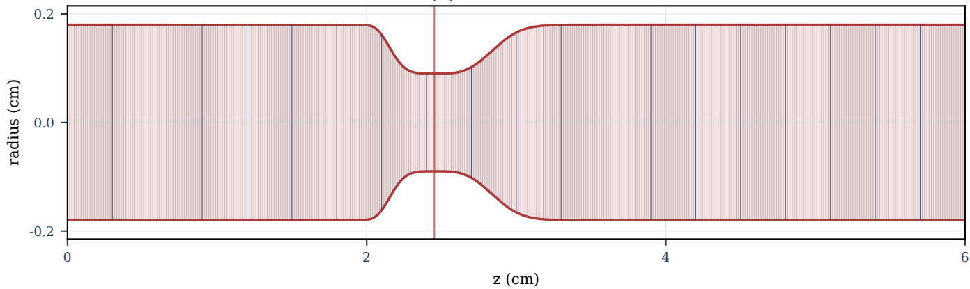
(b) FVM cell mesh
