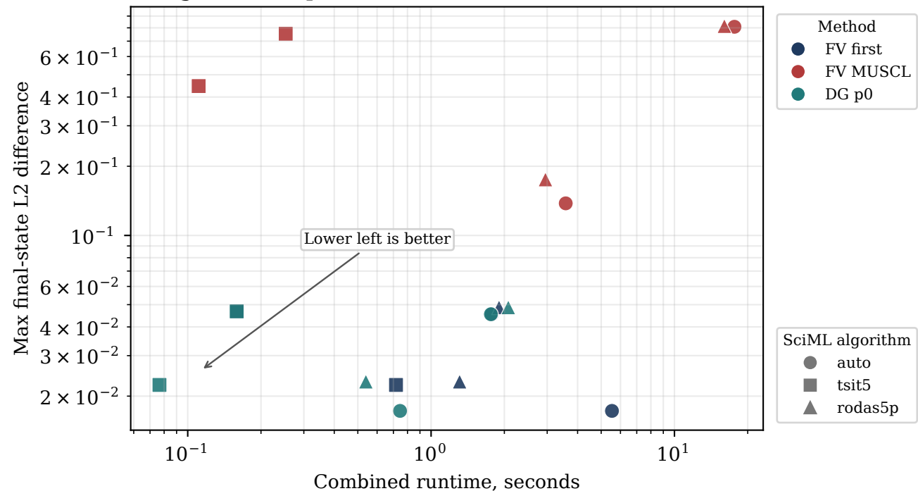
Time-integrator comparison: runtime versus final-state difference
