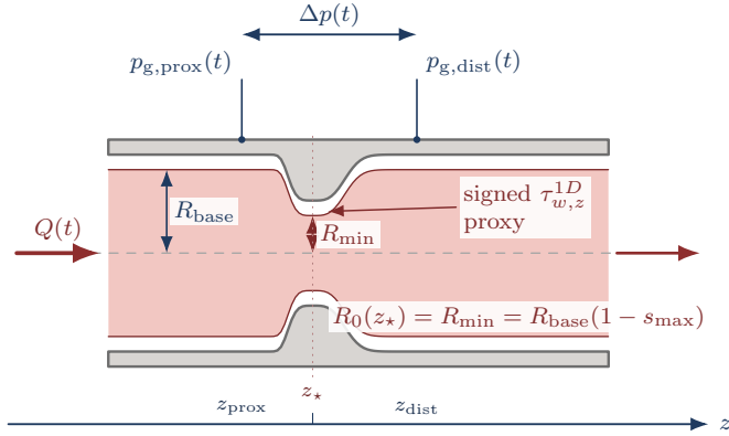
Figure 6: Schematic tap and output convention for an idealized stenosis, not drawn from a computed case. The taps define \Delta p(t) ; Convention C.3 supplies the pressure-ratio observation maps, averaging window, pressure reference, and admissibility rule for \text{PR}_{1D}(\tau_{\text{PR}}) .
