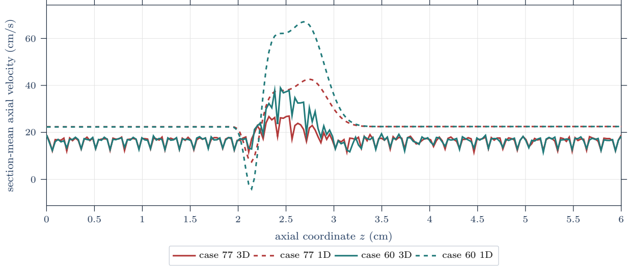
Figure 7: Section-mean axial velocity comparison at T = 1 . Solid curves are resolved 3D node-slab means; dashed curves are interpolated 1D Q/a , equivalently Q_{\text{phys}}/A_{\text{phys}} under the recorded \pi -scaling.
