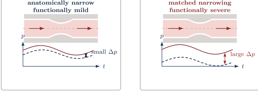
Figure 6: Pressure–flow motivation for reduced pressure outputs. The schematic distinguishes an anatomical narrowing from the pressure-loss signature used by reduced-model outputs.
