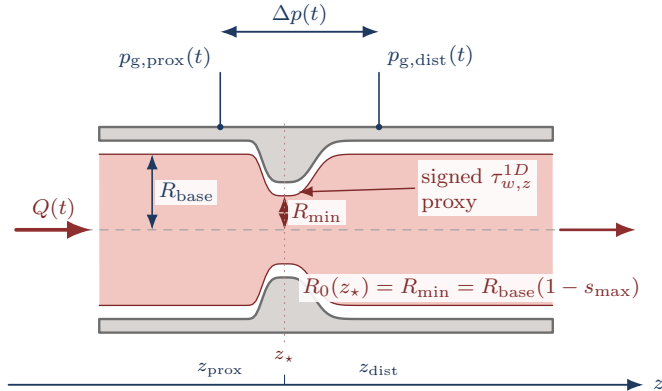
Figure 7: Schematic tap and output convention for an idealized stenosis, not drawn from a computed case. The taps define \Delta p(t) ; Convention C.3 supplies the pressure-ratio observation maps, averaging window, pressure reference, and admissibility rule for \text{PR}_{1D}(\pi_{\text{PR}}) .
