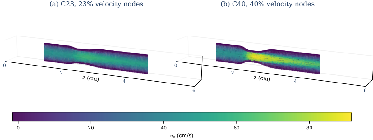
Figure 11: Resolved 3D node-centered axial velocity fields for the two T = 1 comparison cases used in Section 5. Panel (a) shows C23 with 22,691 loaded nodes; panel (b) shows C40 with 21,975 loaded nodes. The shared color scale makes the stronger axial-velocity concentration in C40 visible. Sparse arrows indicate local vector direction, and the transparent surface frames the 3D point cloud. These are resolved velocity comparison-data renderings, not the stationary-Stokes pathline proxy or a pressure-drop, FFR, or patient-specific clinical calibration measurement.
