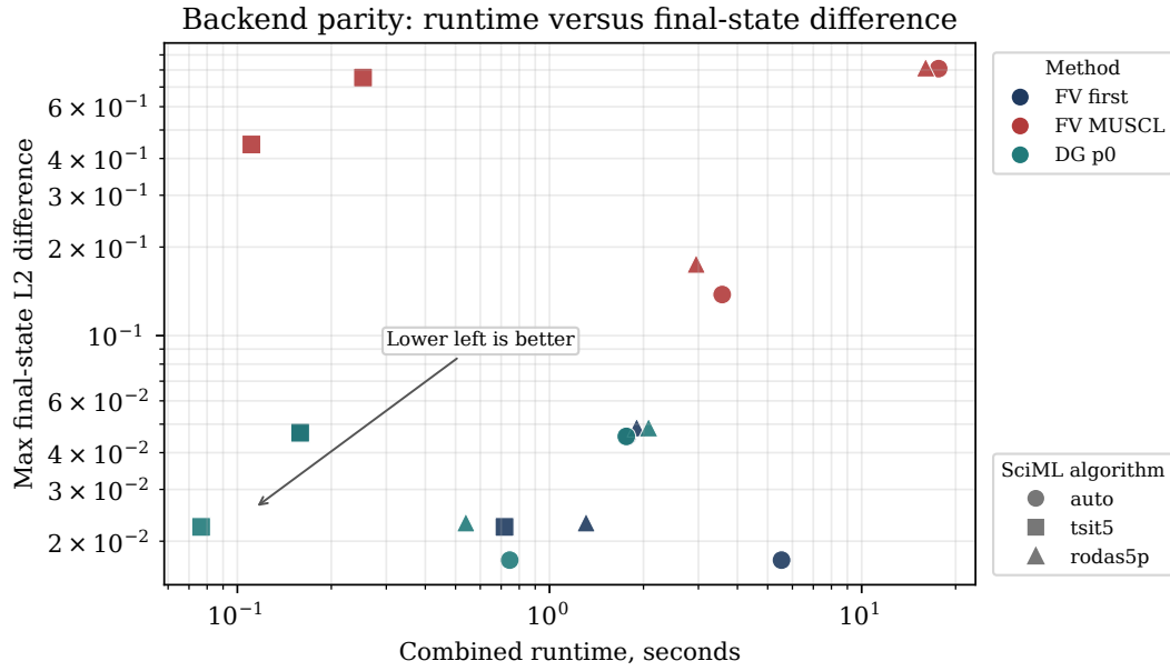
Figure 8: Native/SciML cross-integrator discrepancy versus runtime for compatible methods. The native path uses the stagewise positivity limiter; the SciML path integrates the unprojected semi-discrete system. The figure is therefore a cross-integrator diagnostic, not a proof of solver equivalence.
