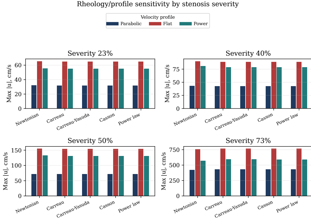
Figure 10: Rheology/profile sensitivity summary for declared descriptor combinations. This stage checks descriptor plumbing and response direction; it is not part of the principal C23/C40 comparison evidence.
