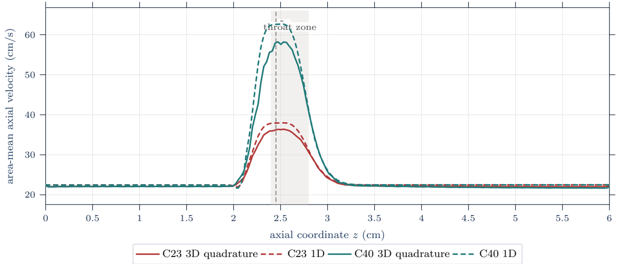
Figure 12: Area-mean axial velocity comparison at t = 1.0 s. Solid curves are tetrahedral cross-section quadrature means from the resolved 3D velocity field; dashed curves are interpolated 1D means \bar{u} = q/a = Q_{\text{phys}}/A_{\text{phys}} . The shaded band marks the throat-centered stenosis region.
