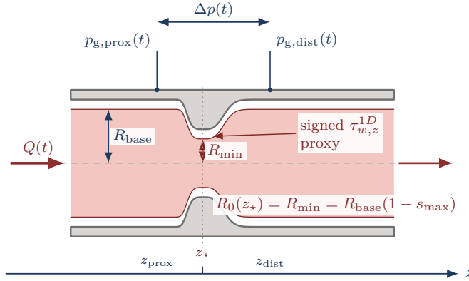
Figure 7: Schematic tap and output convention for an idealized stenosis, not drawn from a computed case. The taps define \Delta p(t) ; Convention C.3 supplies the pressure-ratio observation maps, averaging window, pressure reference, and admissibility rule for \text{PR}_{1D}(\pi_{\text{PR}}) .
