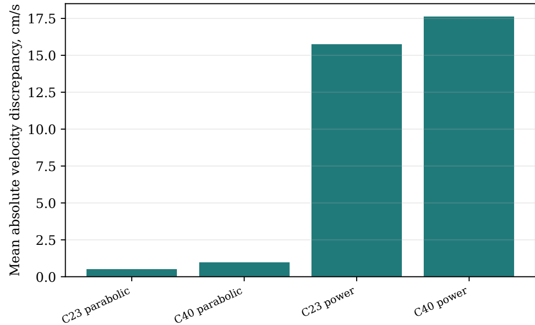
Resolved-velocity CrossSectionQuadratureOperator diagnostic
