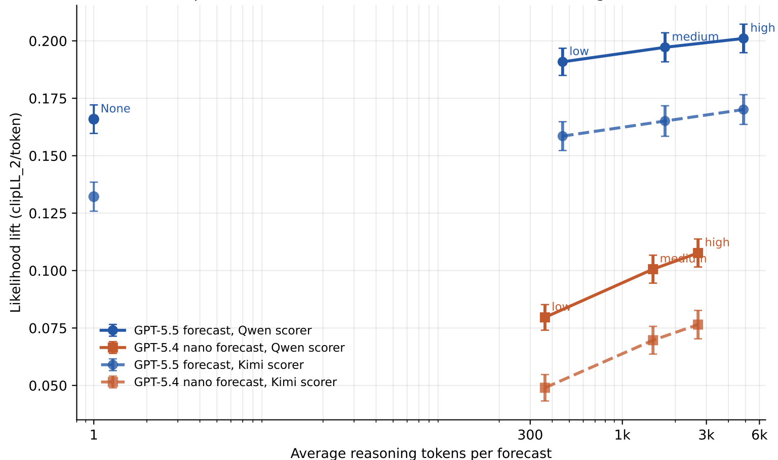
Equation-suffix forecasts: likelihood lift vs. reasoning tokens
