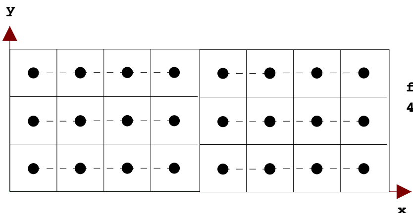
d) Layout with 12 threads running on a single node, with periodic boundaries: ((4,2)P, (3,2)P)
