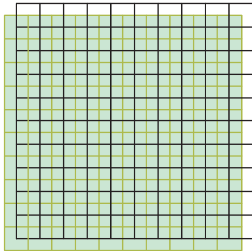
Global grid
