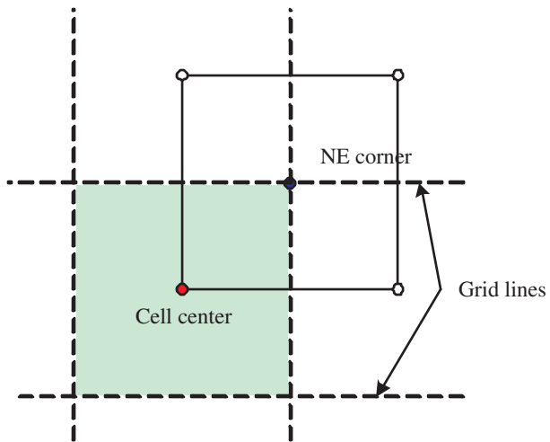
Computational cell
