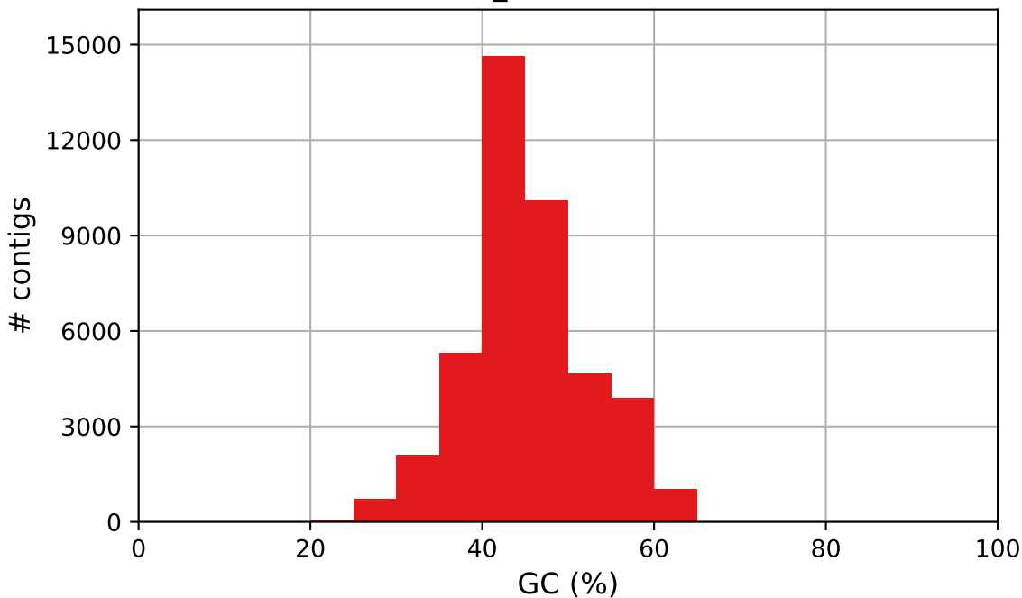
ERR011348_MEGAHIT GC content
