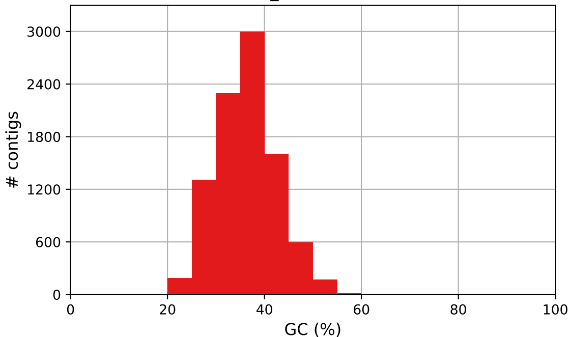
ERR011349_MEGAHIT GC content
