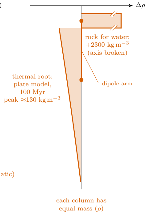
(c) \Delta\rho(z) : ridge – isostatic
