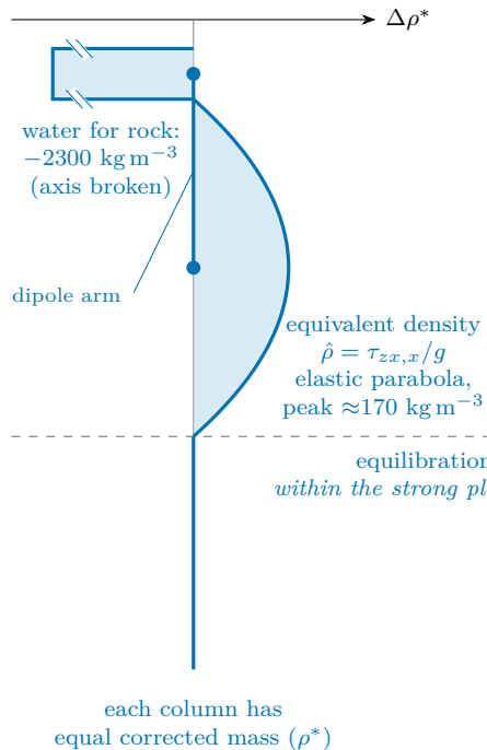
(a) \Delta\rho^*(z) : trench – isostatic
