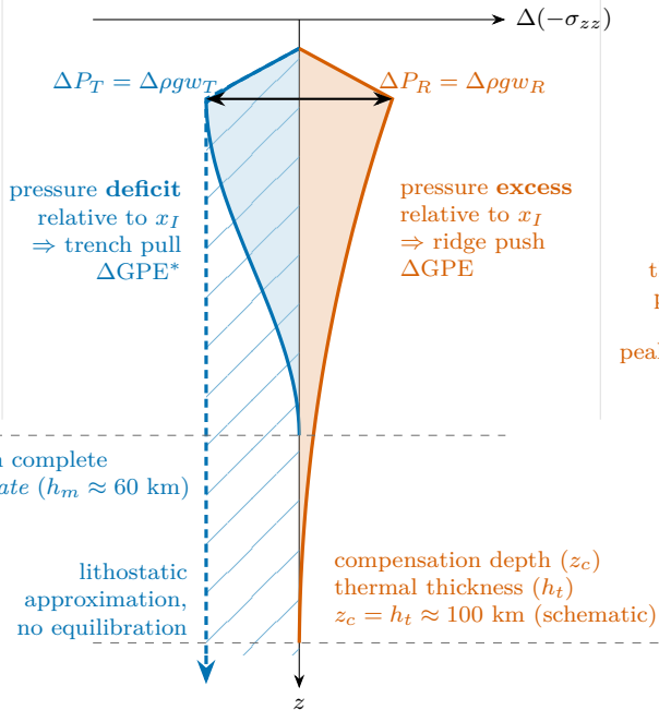
(b) topographic pressure anomaly \Delta(-\sigma_{zz})(z) , relative to the same isostatic column
