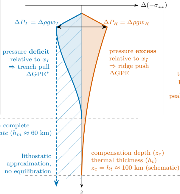
(b) topographic pressure anomaly \Delta(-\sigma_{zz})(z) , relative to the same isostatic column
