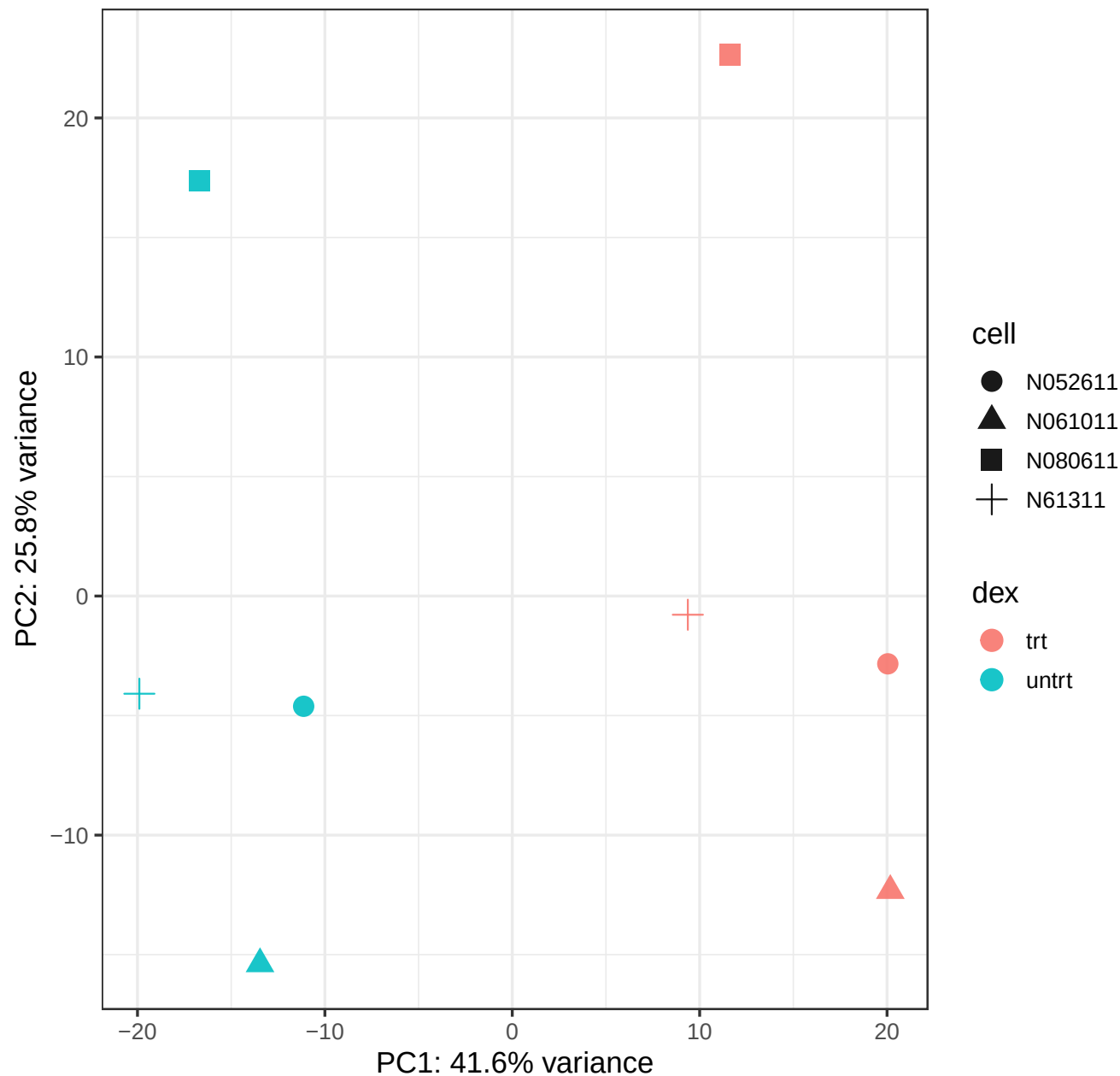
PCA of variance-stabilized counts (top 500 variable genes)
