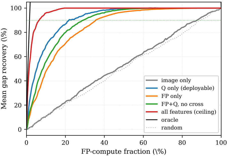
Feature-subset ablation, W4-channel LOO (16 ViT-L/16 tasks)
