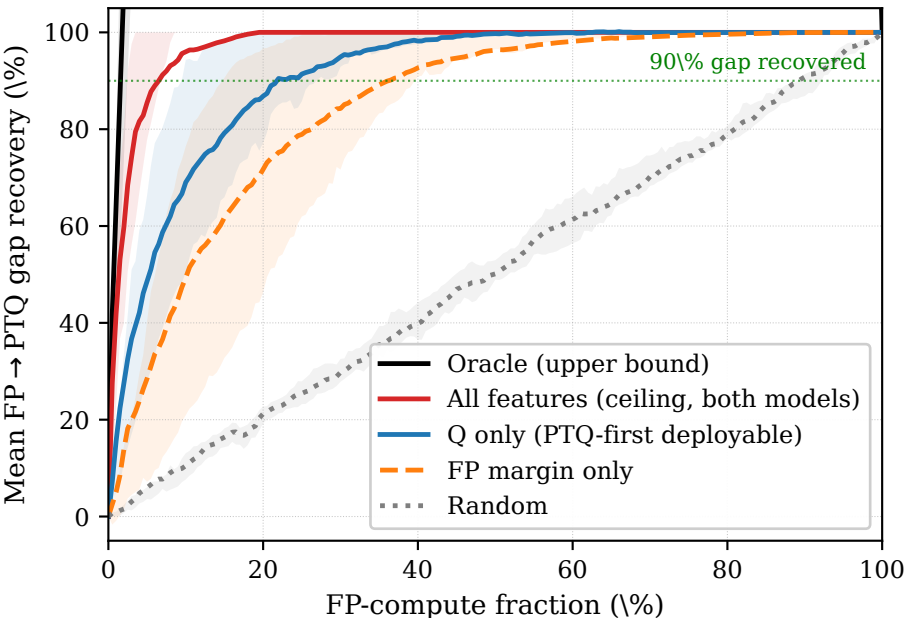
LOO cross-task routing at W4-channel (16 ViT-L/16 tasks)
