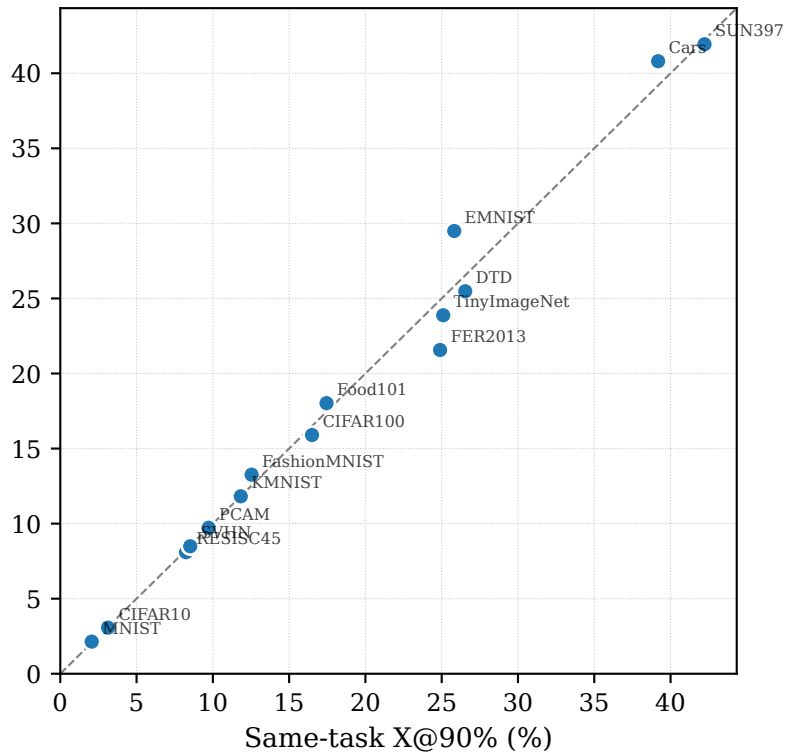
ViT-L/16 --- W4-channel (15 tasks)
