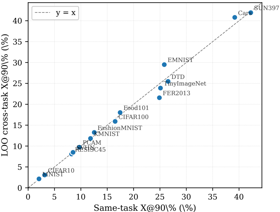
Q-only deployable LOO vs same-task X@90\% (W4-channel, 15 ViT-L/16 tasks)
