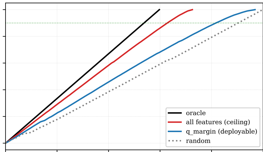
ViT-L/16 --- W3-channel (catastrophic) (21 tasks)
