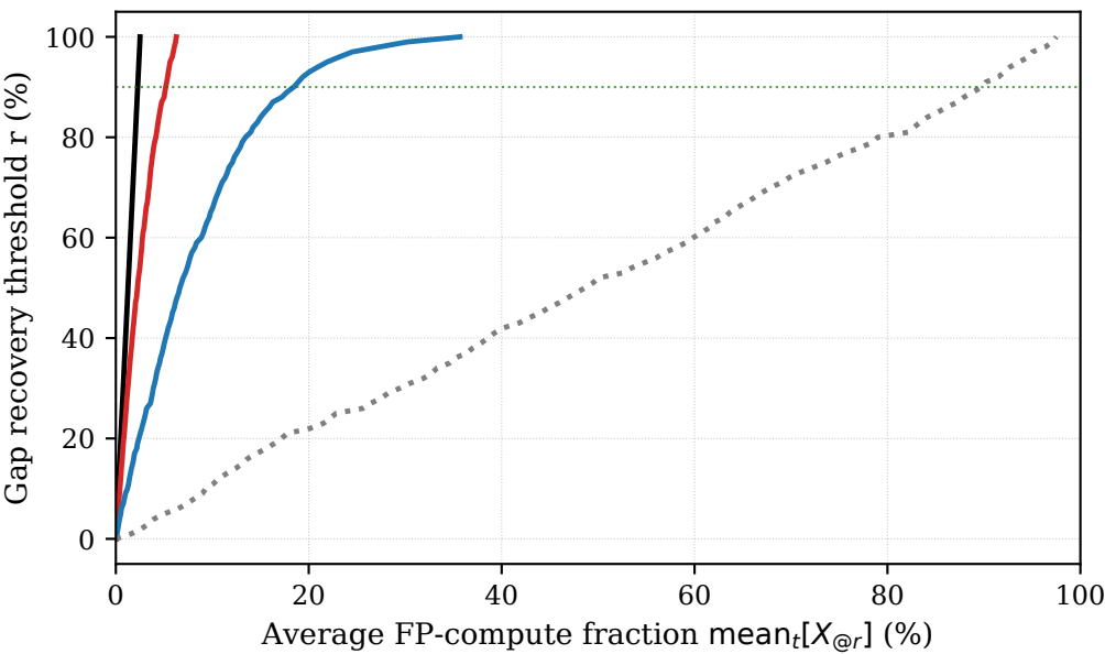
ViT-L/16 --- W4-channel (recoverable) (16 tasks)
