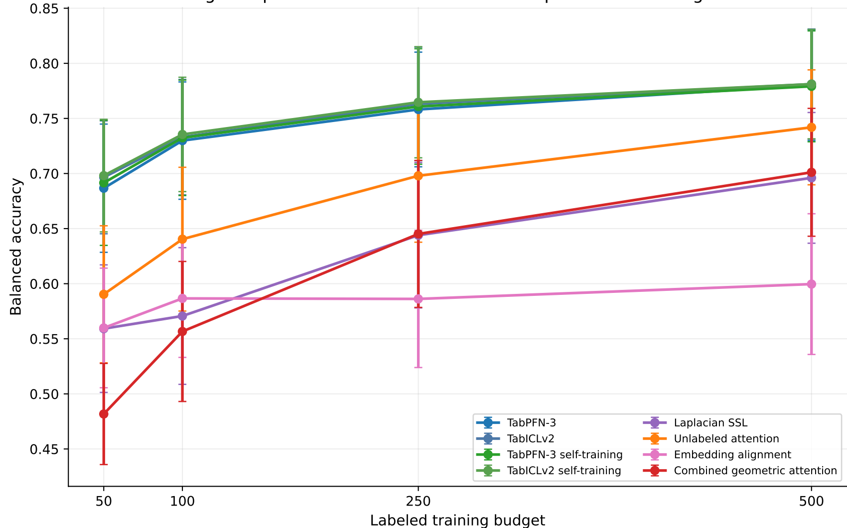
Eight requested methods across the complete 10-dataset grid
